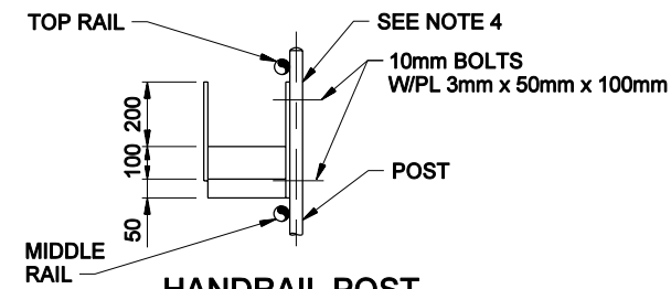
HANDRAIL POST MOUNTED
