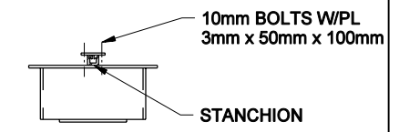
STANCHION MOUNTED
