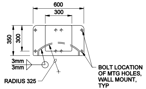
WALL MOUNTED
