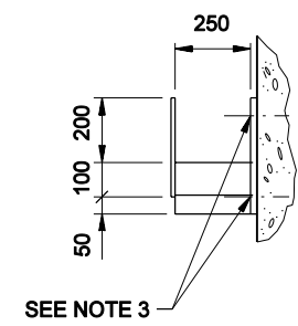
STANCHION MOUNTED
